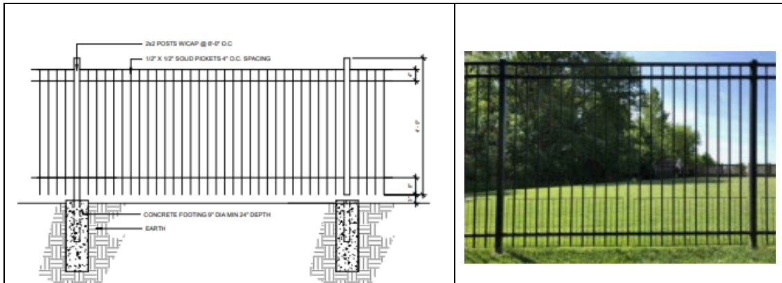
Proposed 4-foot Fence
